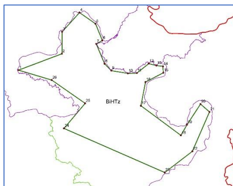
Fig.4 Exploration block BiHTz (Area =1511 km 2 )
