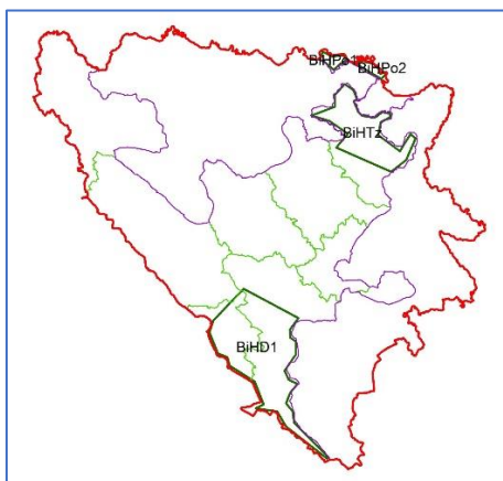
Fig.1 Map of FBiH exploration blocks
